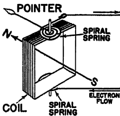
Meter movement.
